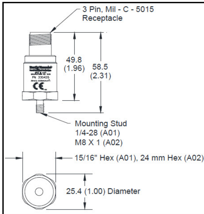
Figure 5: 330400/330425 Accelerometer Sensor
