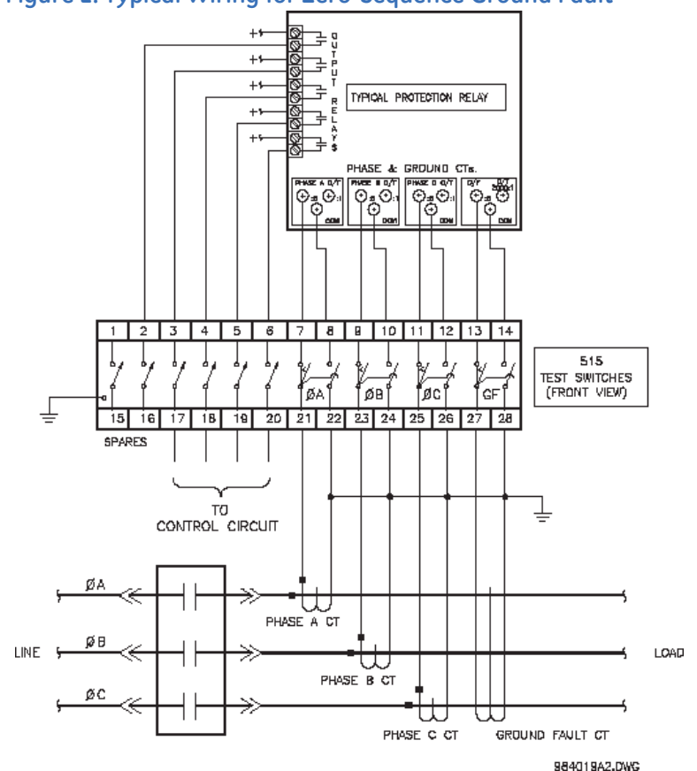
Figure 2: Typical Wiring for Zero-Sequence Ground Fault
