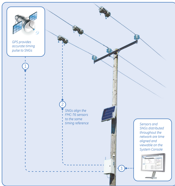
Typical feeder measurement installation
