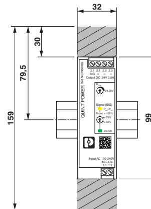
Dimensional drawing
