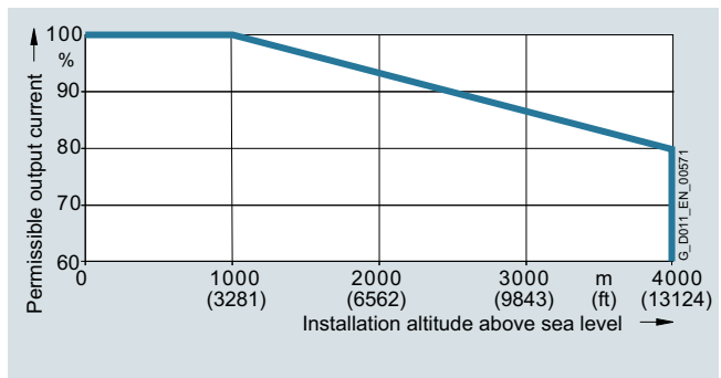
Permissible output current as a function of installation altitude for SINAMICS G120X for low overload (LO)
