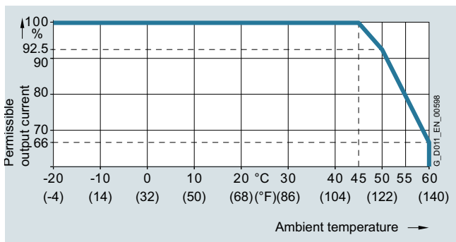
Permissible output current as a function of ambient temperature for SINAMICS G120X, frame sizes FSA to FSG, for low overload (LO)
