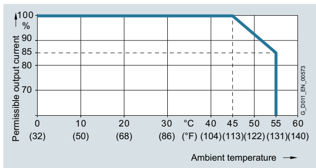
Permissible output current as a function of ambient temperature for SINAMICS G120X, frame sizes FSH and FSJ, for low overload (LO)
